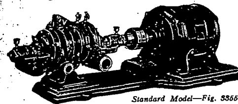
Standard Model—Fig. 3356
