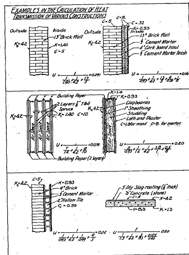
FIG. 3. COMPUTING HEAT TRANSMISSION COEFFICIENTS FOR BUILDING WALLS.
