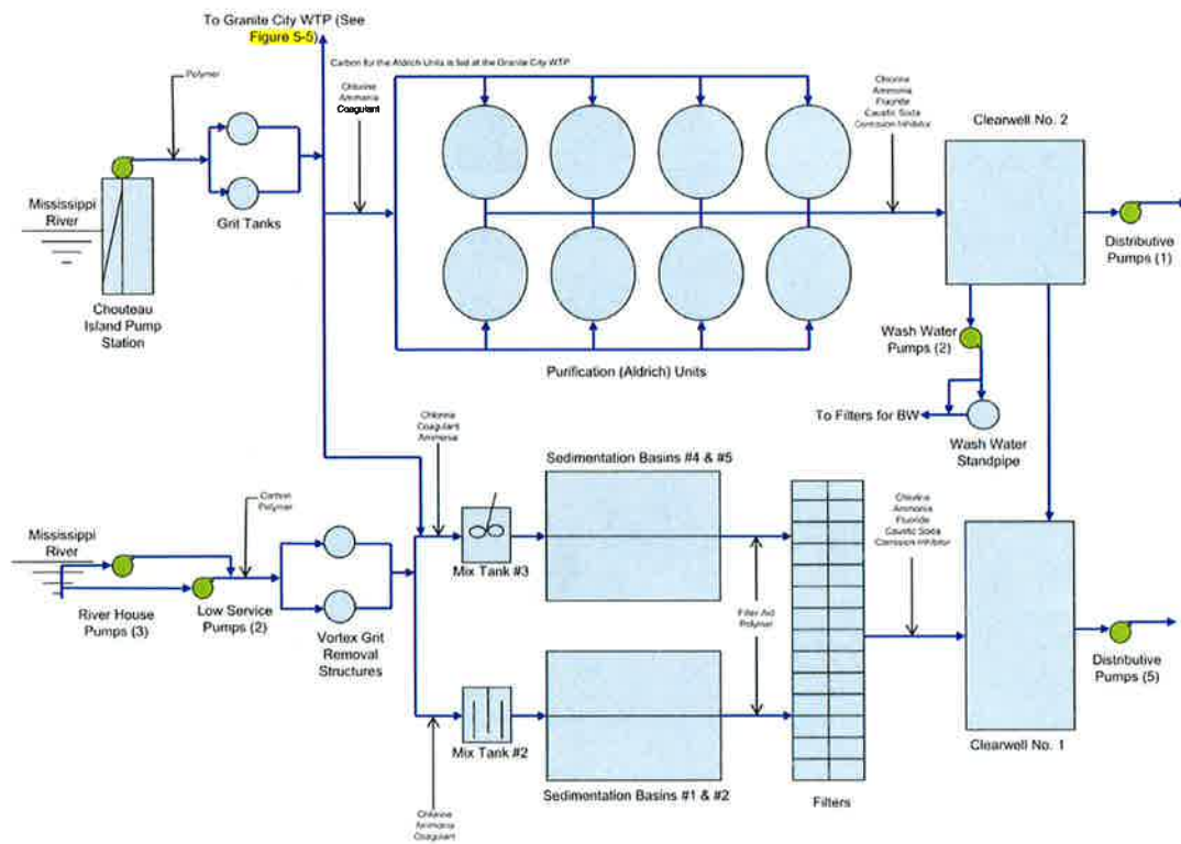
Exhibit 4-12 Schematic of ESLWTP
