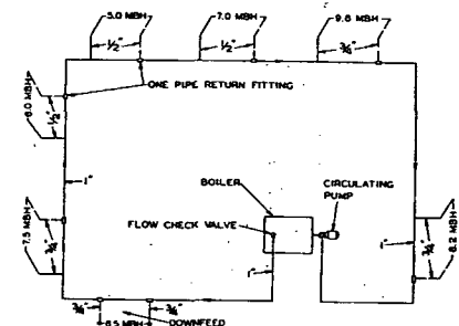
Fig. 10.... A One-Pipe System
