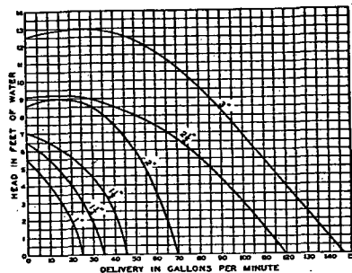
Fig. 9.... Performance Chart for Circulating Pump
