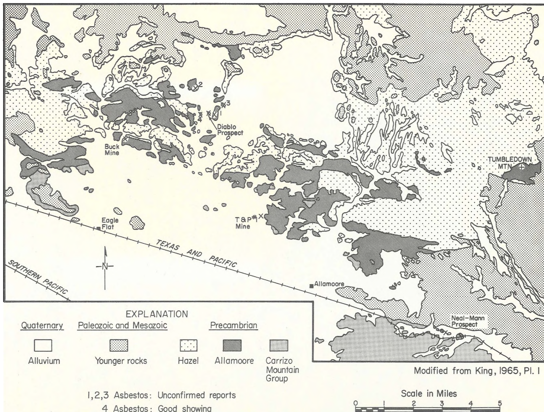
FIG. 1. General geology and asbestos deposits, Allamoore talc district.
