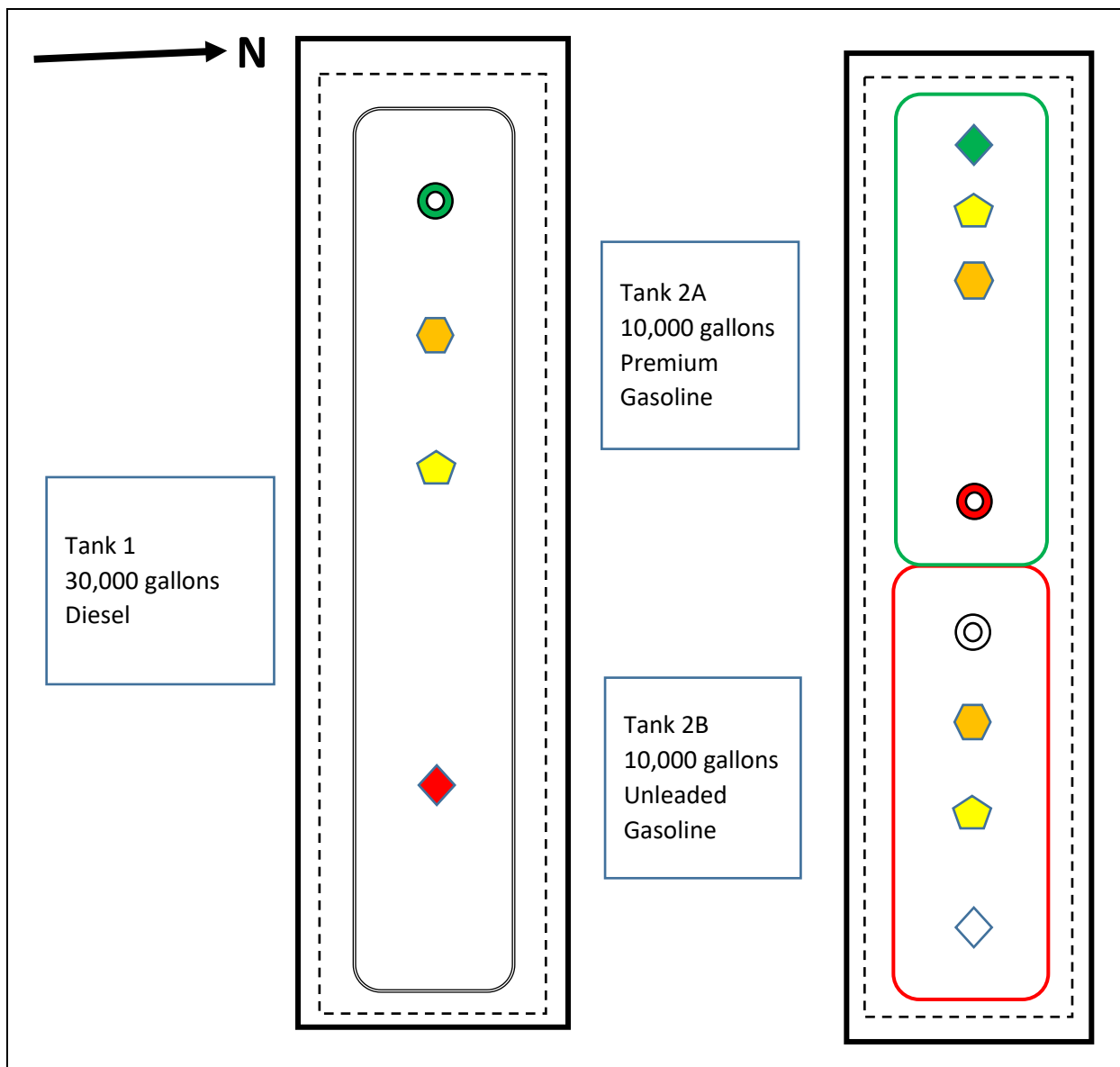
FIGURE 2 – TANK DIAGRAM
