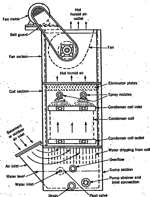
FIG. 10. SCHEMATIC VIEW OF AN EVAPORATIVE CONDENSER
