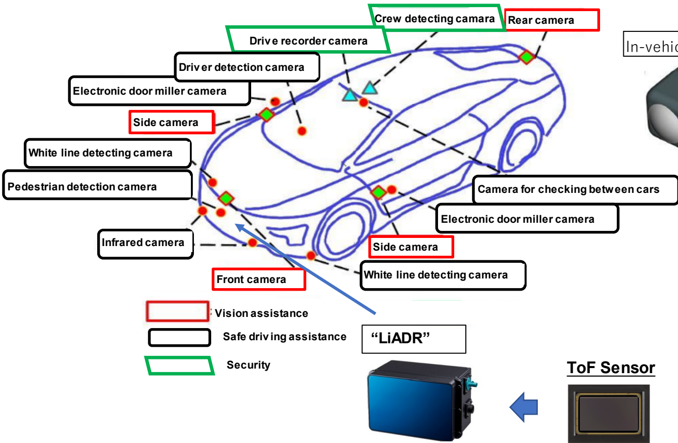
On-board camera position and function
