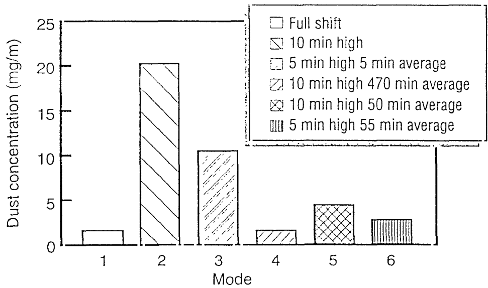
Figure 122 COMPARISON OF SAMPLING TECHNIQUES AND REGISTERING OF HIGH DUST LEVELS
