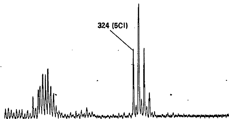
Herring oil mass spectrum of peak 4
