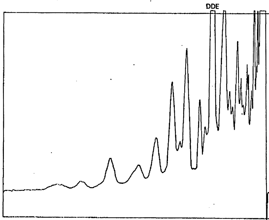
Fig 3 G.L.C.-E.C. Chromatogram Herring oil extract
