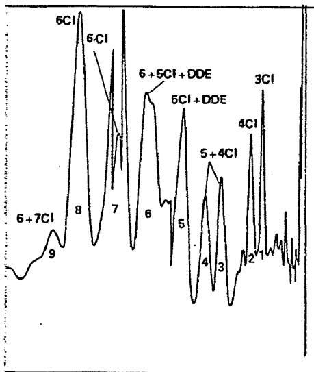
Fig 8 Heron egg F.I.D.-M.S. split
