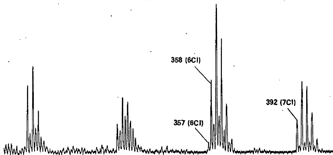
Herring oil mass spectrum of peak 10
