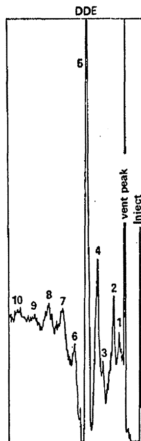
Fig 6 G.L.C.-M.C. Chromatogram Herring oil extract
