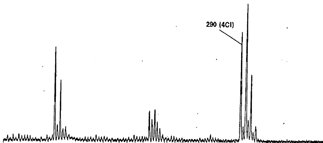
Heron egg mass spectrum of peak 2
