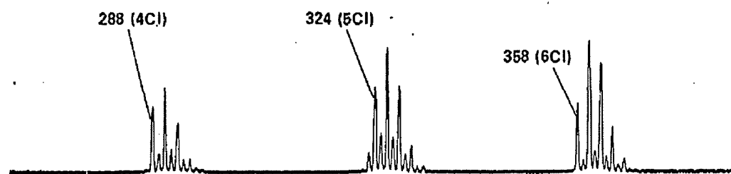
Aroclor 1254 mass spectrum of peak 9
