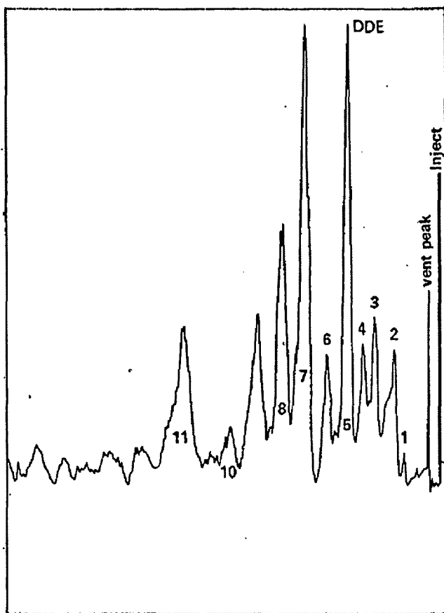
Fig 5 G.L.C.-M.C. Chromatogram Heron egg extract
