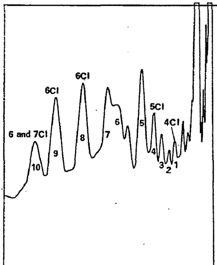
Fig 9 Herring oil F.I.D.-M.S. split
