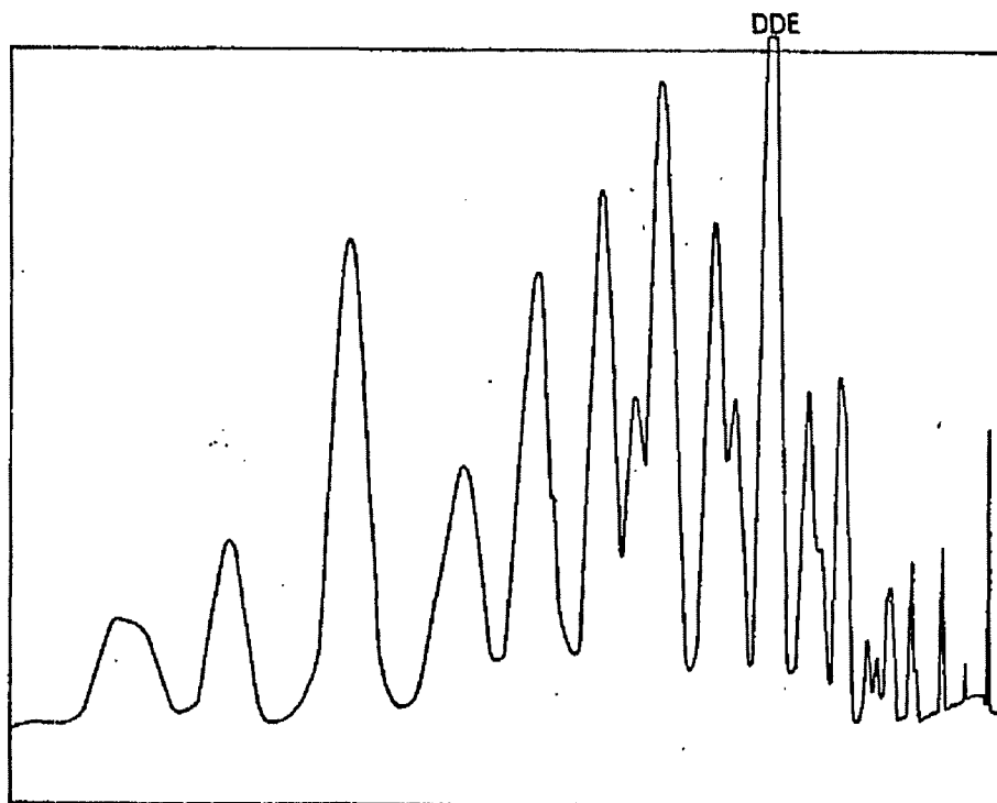
Fig 2 G.L.C.-E.C. Chromatogram Heron egg extract
