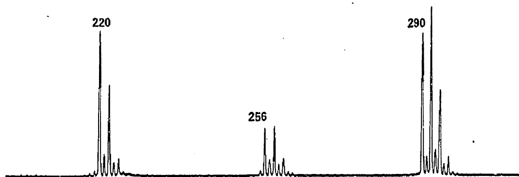
Aroclor 1254 mass spectrum of peak 2
