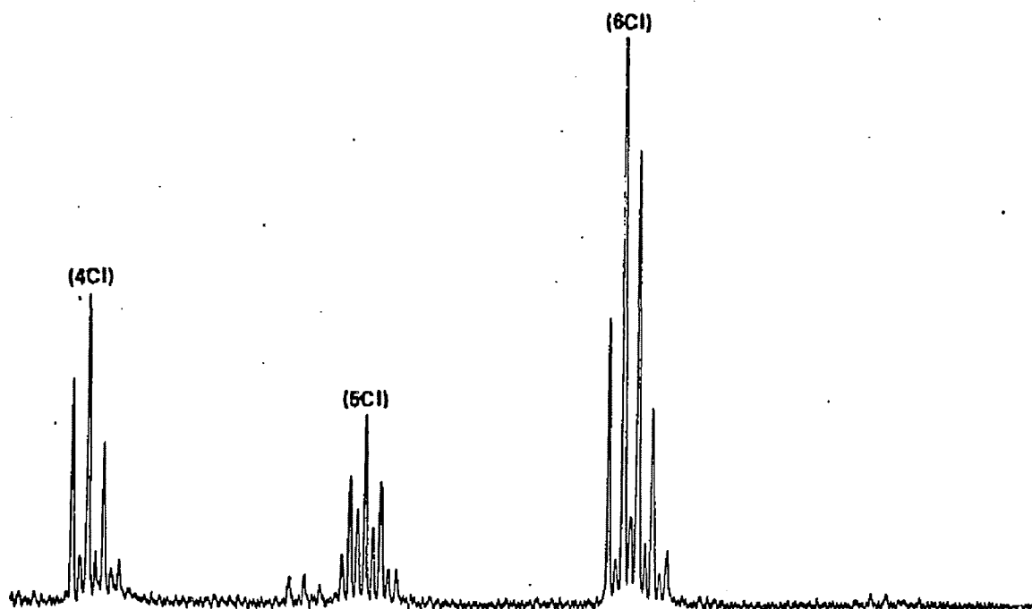
Heron egg mass spectrum of peak 8
