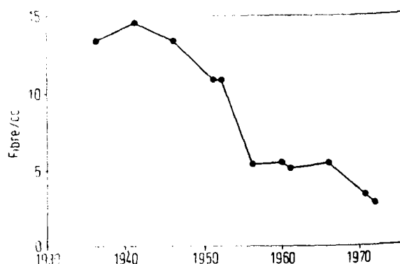
Fig. 4—Average dust levels, weighted by the number of men at each level, in an asbestos textile factory, 1936–72.
