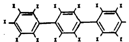
Polychlorinated Terphenyls
