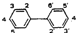
BIPHENYL MOLECULE AND RING NUMBERING SYSTEM
