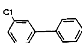
3-chlorobiphenyl
