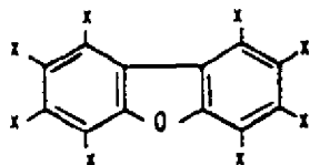
Chlorinated Dibenzofurans
