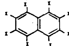
Polychlorinated Naphthalenes
