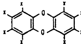
Chlorinated Dibenzodioxin
