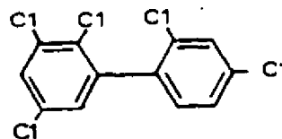
2,2',3,4',5-pentachlorobiphenyl
