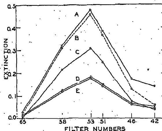
Figure 5. Detection of 4-Chloro-3,5-dinitrobenzoic Acid
