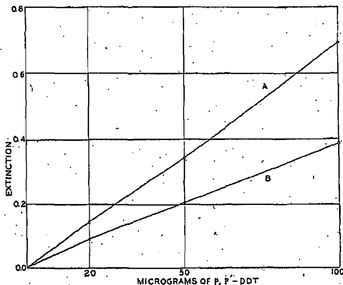
Figure 3. Analytical Calibration Curves for p,p' -DDT
