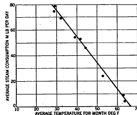
FIG. 1. METHOD OF DETERMINING BASE TEMPERATURE FOR DEGREE-DAY CALCULATIONS 5
