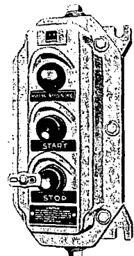
Three Element NEMA Type 7D-9EFG Enclosure
