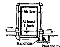
FIG. 29. LOOPING DRY RETURN MAIN AROUND OPENING
