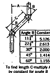
FIG. 31. CONSTANTS FOR DETERMINING LENGTH OFFSET PIPE
