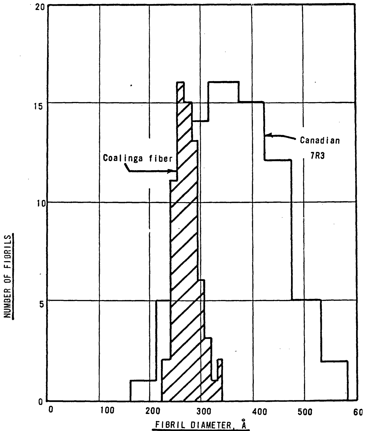
HISTOGRAM OF A TYPICAL FIBRIL DIAMETER DISTRIBUTION
