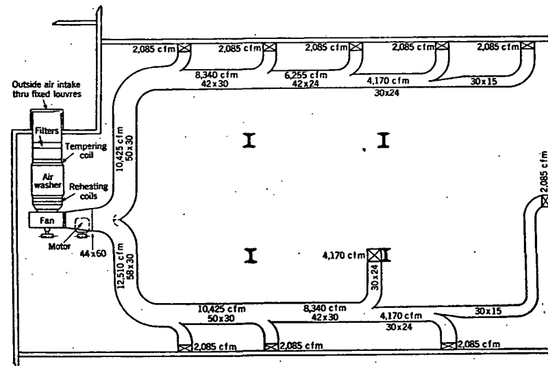
FIG. 7. TYPICAL LAYOUT OF AIR DISTRIBUTION SYSTEM
