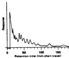
Fig. 7. Gas chromatogram of a 10- \mu l aliquot of extract (1 ml) obtained from 42-day compost (sample 11 in Table I)
