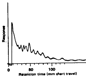
Fig. 5. Gas chromatogram of a 10- \mu l aliquot of extract (1 ml) obtained from incinerator residue fines (sample 4 in Table I)
