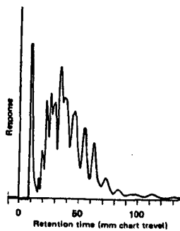
Fig. 2. Gas chromatogram of 50 ng of Arochlor 1248
