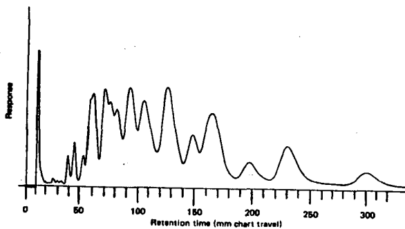
Fig. 4. Gas chromatogram of 50 ng of Arochlor 1262
