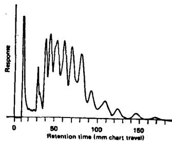
Fig. 3. Gas chromatogram of 40 ng of Arochlor 1254
