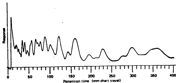
Fig. 6. Gas chromatogram of a 10- \mu l aliquot of extract (1 ml) obtained from incinerator fly ash (sample 7 in Table I)
