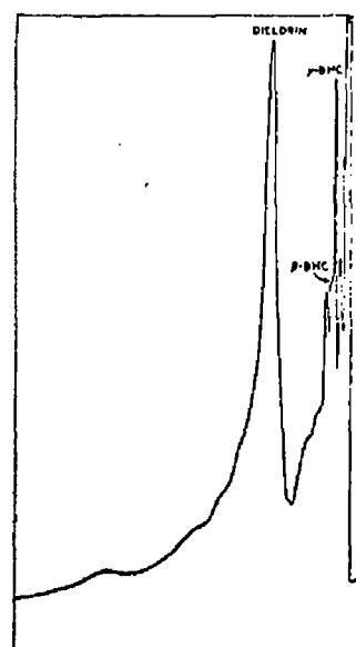
Fig. 4. Gas-liquid chromatogram from section 5 of the thin-layer chromatoplate
