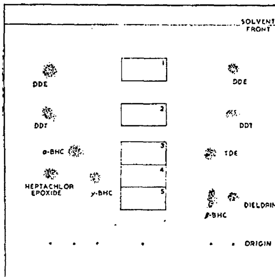
Fig. 1. Thin-layer chromatoplate
