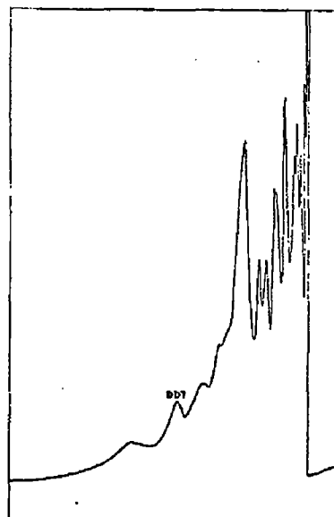
Fig. 3. Gas-liquid chromatogram from section 2 of the thin-layer chromatoplate
