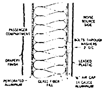
FIGURE 7. Section through the sound barrier used in HS Denison. It is basically similar to that used in the stationary turbine (Figure 4) except that heavier leaded vinyl sheet is employed and it is paint-suspended for maximum limpness.
