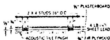
FIGURE 9. Section through the wall employed in the Franklin Institute test room. The original drywall (gypsum board face and wood stud framing) existed and the lead and finish were added.
