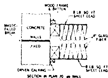
FIGURE 11. Section through the 70-db wall.
