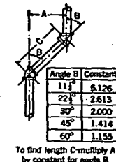
FIG. 38. CONSTANTS FOR DETERMINING LENGTH OF OFFSET PIPE
