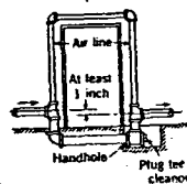
FIG. 36. LOOPING DRY RETURN MAIN AROUND OPENING
