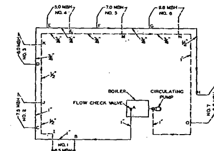
Fig. 8.... A Two-Pipe Reversed-Return System
