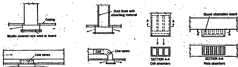
FIG. 8. OUTLET CELLS FOR FAN OUTLETS OR GRILLES
