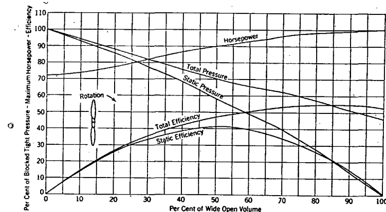
FIG. 2. OPERATING CHARACTERISTICS OF AN AIRPLANE PROPELLER FAN
