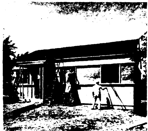
Phenol plywood was used for interior and exterior walls and roof sheathing. Hard sheet lead formed the chimney flashing.
