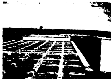
Three views of the "honey comb" acoustical block towers with lead flashing and copings at the Engine Test Building of the Sacramento Air Depot.
