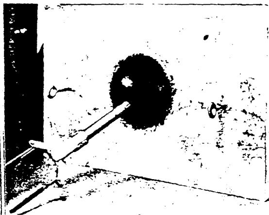
The construction of a radiation-shielded, ball-joint socket for the Argonne National Laboratory mobile shield presented a problem. It was solved, at low cost, by the development of a cold-setting lead cement that could be poured into easily constructed wooden forms around the ball itself.
