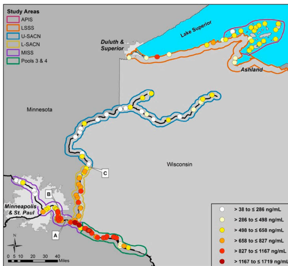
Figure 2. Geometric mean concentrations of \Sigma PFCs in bald eagle nestlings, 2006–2011. Values are modeled from measurements by three independent laboratories. Categories were selected using natural breaks in Arc GIS. A = location of 3M PFC production facility; B = Minneapolis/St. Paul WWTP and St. Paul Downtown Airport; C = the communities of St. Croix Falls, WI and Taylors Falls, MN. See Figure 1 for study area acronyms.
