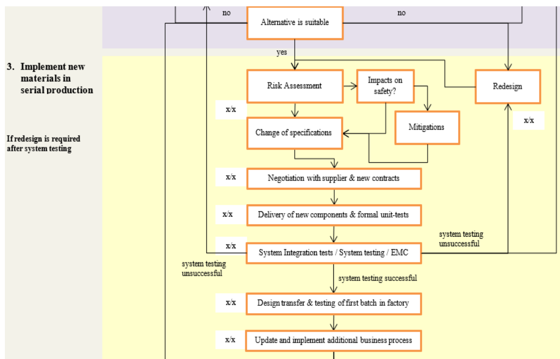
Figure 12: Flowchart step 3: Implementation in serial production.
