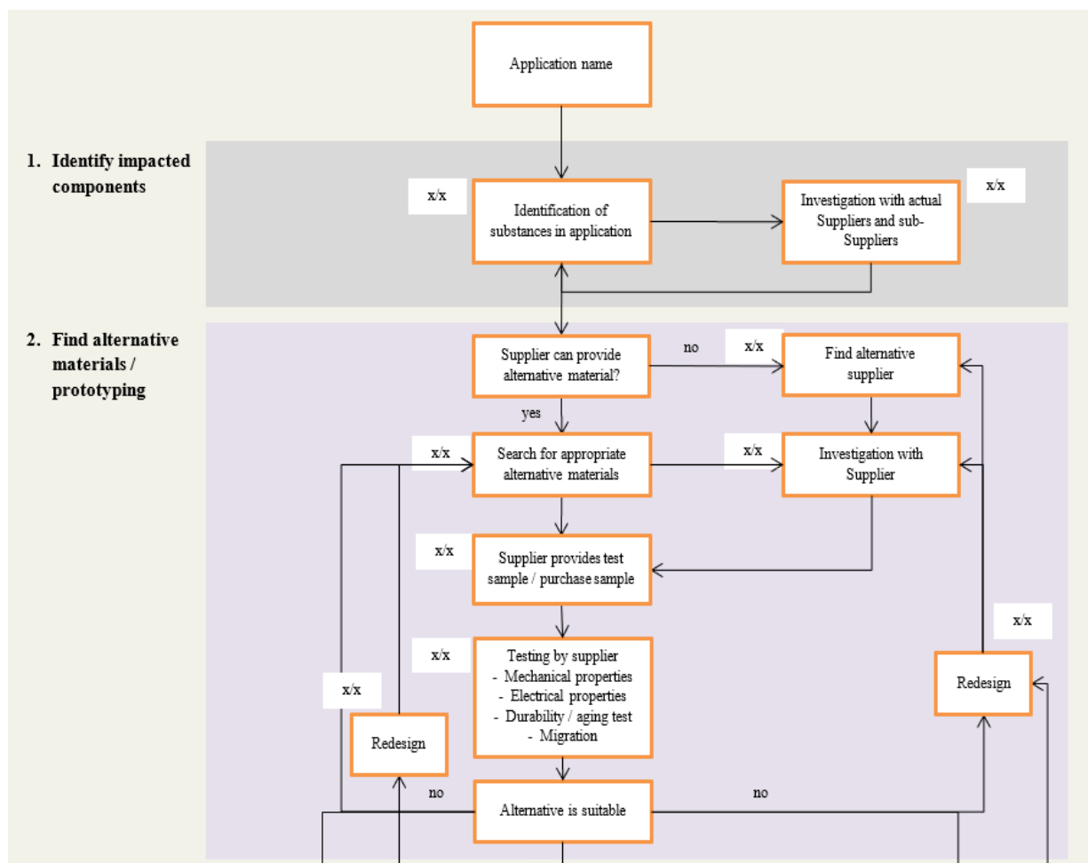
Figure 11: Flowchart steps 1 & 2: Identifying alternatives working with suppliers prototyping and testing of new components
