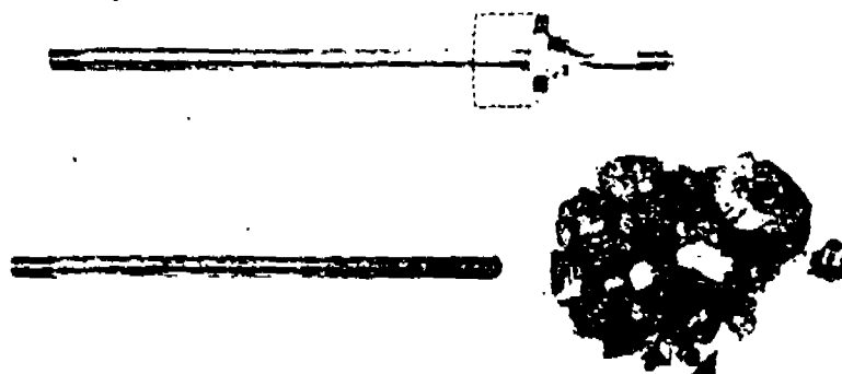
Fig. 3. Ignition of titanium poppet.
