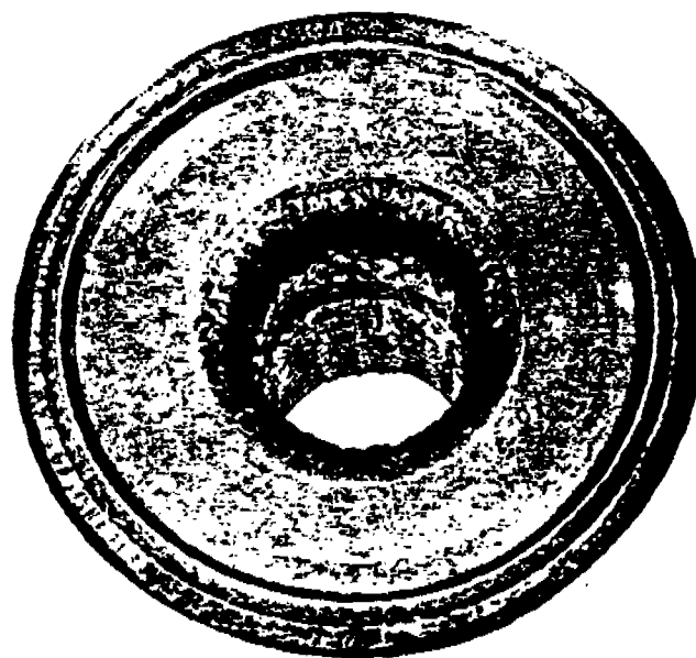
Fig. 9. Rupture disk after reaction.
