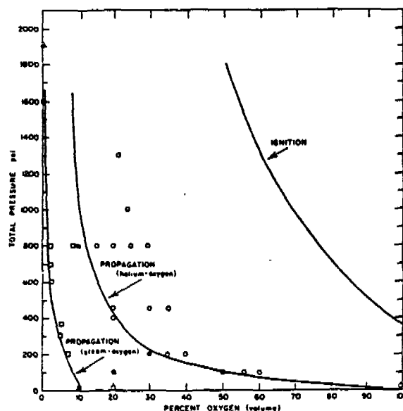
Fig. 10. Ignition propagation in helium-oxygen and steam-oxygen mixtures.
