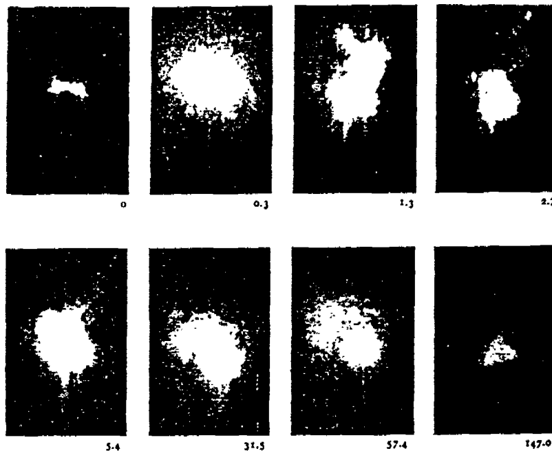
Fig. 5. Ignition of titanium rod.
