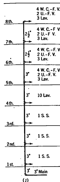
FIG. 5. UP-FEED SYSTEM
