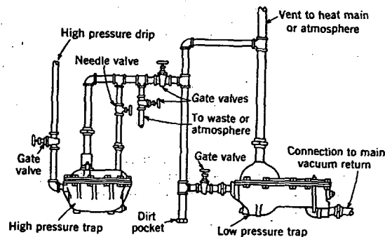
FIG. 17. METHOD OF DISCHARGING HIGH-PRESSURE APPARATUS INTO LOW-PRESSURE HEATING MAINS AND VACUUM RETURN MAINS THROUGH A LOW-PRESSURE TRAP
