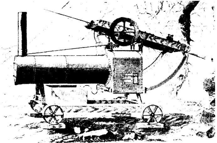
THE FIRST PERCUSSION ROCK DRILL EVER MADE.
