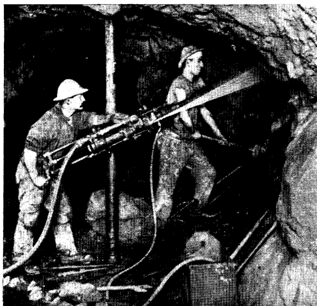
PLATE XII.—Rock drill of 1902 with spray—drifting.
