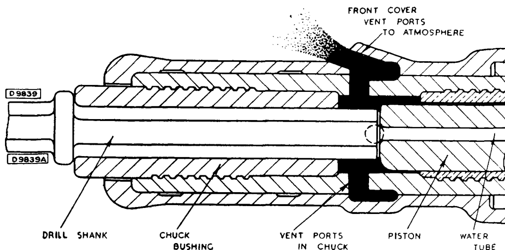
PLATE XXIV.—Modern vented front head.
