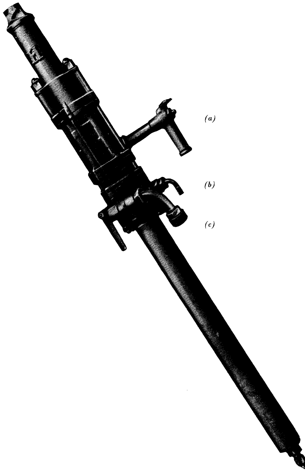
PLATE XXX.—Automatic overhand stopper with axial water tube : (a) control handle ; (b) connexion for water hose ; (c) connexion for air hose.
