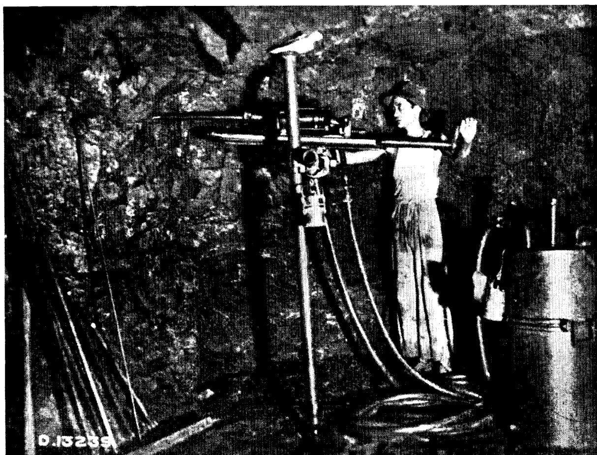
PLATE XVI.—Cradle-mounted hand drill drifting in a Malayan mine. (Note tank for supplying water under pressure.)
