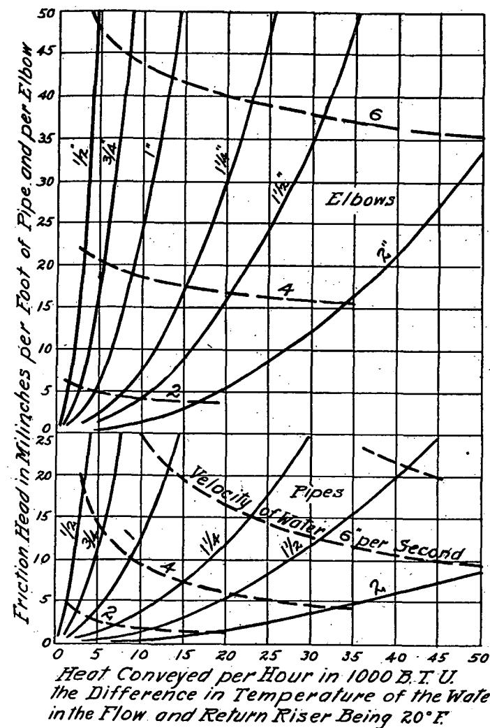
FIG. 7. FRICTION HEADS, IN PIPES AND ELBOWS, FOR A 20 DEG. TEMPERATURE DIFFERENCE OF THE WATER IN THE FLOW AND RETURN LINES
