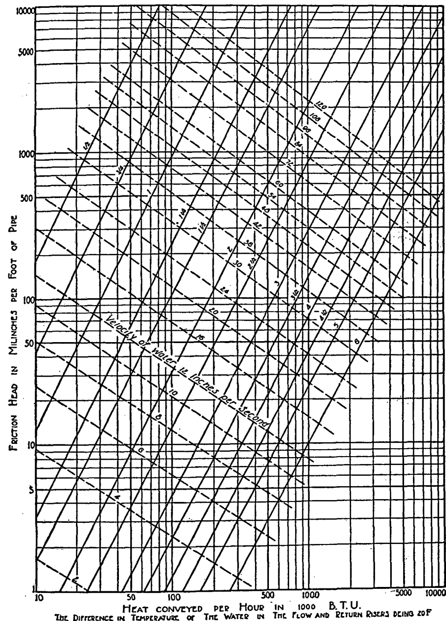
FIG. 4. FRICTION HEADS IN PIPES FOR A 20 DEG. TEMPERATURE DIFFERENCE OF THE WATER IN THE FLOW AND RETURN LINES
