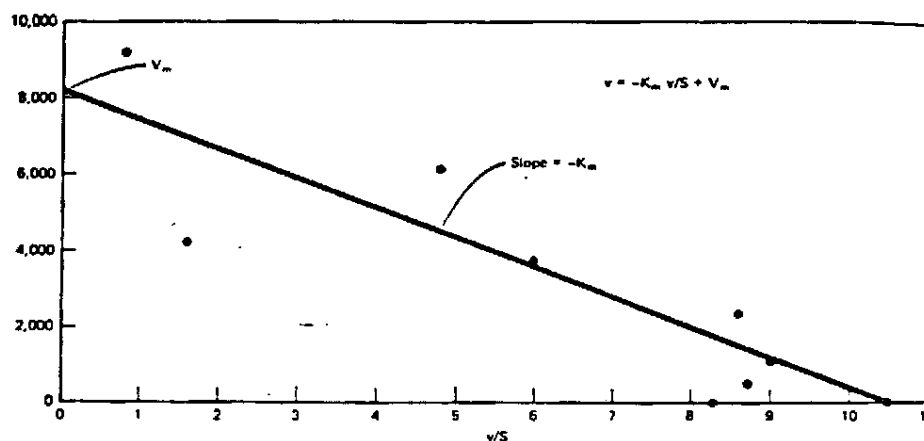
FIG. 1. Metabolism of vinyl chloride analyzed in accordance with the Woolf-Augustinsson-Hofstee linearized form of the Michaelis-Menten equation. Values of v and v/S were taken from Table 1. The line was fit by linear regression analysis. The correlation coefficient, R , was 0.88.
