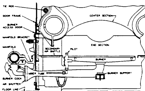
FIG. 8—Burner and Auxiliary Pilot
