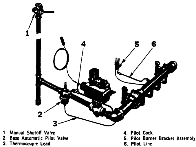
FIG. 18—Control Connections
