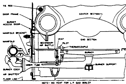
FIG. 7—Burner No. 2 and Pilot Installation-Manual Ignition
