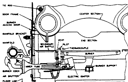
FIG. 6—Burner No. 2 and Pilot Installation-Electric Ignition
