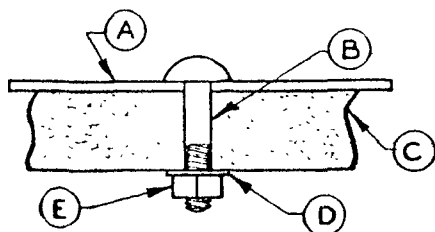
FIGURE 7. Insulation attached by bolts through drilled holes.
