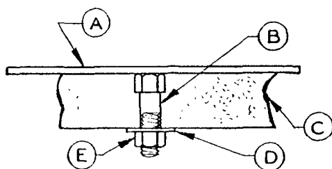
FIGURE 6. Insulation attached by bolts with heads welded to metal surface.
