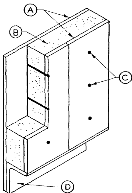
FIGURE 1. Insulation enclosed between metal sheets.
