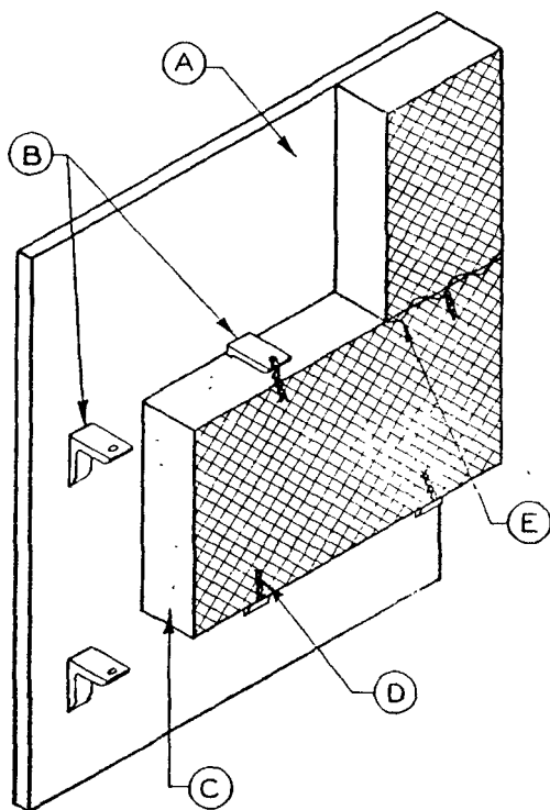
FIGURE 3. Blanket insulation supported by clip angles.
