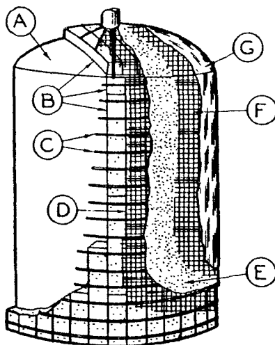
FIGURE 14. Application of mineral wool block insulation on curved surfaces.
