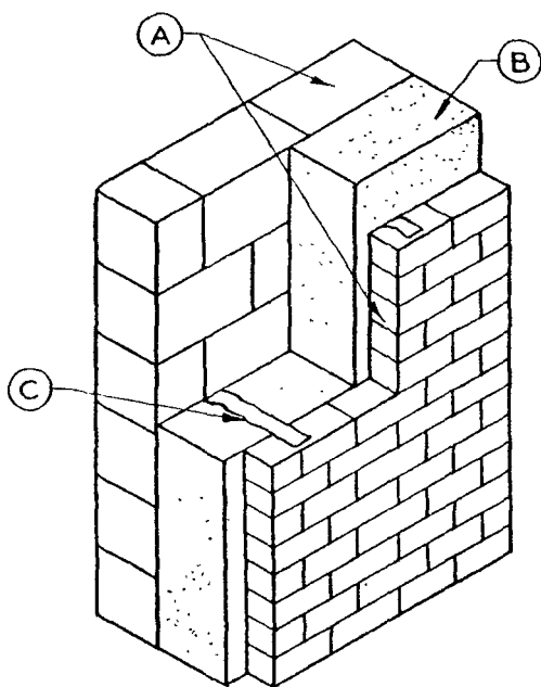
FIGURE 2. Insulation enclosed between masonry walls.
