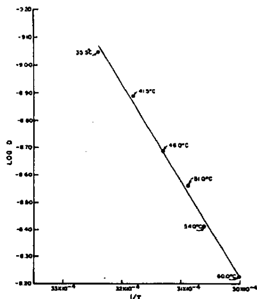
Fig. 18.—A plot of the log of D vs. the reciprocal of the absolute temperature for salicylic acid in nylon. [From Kapadia, A. J., Guess, W. L., and Autian, J., "Sorption and Diffusion Studies of Salicylic Acid in a Nylon Sheet," to be published.]
