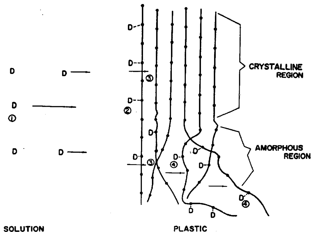
Fig. 10.—A schematic model showing sorption of a drug by nylon. D = drug molecule; --- = polymer chain; and • = binding sites in polymer.
