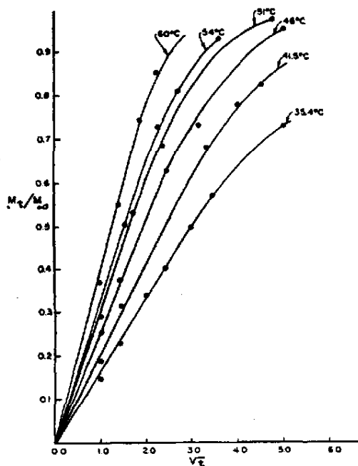
Fig. 11.—Fractional uptake of salicylic acid vs. square root of time at various temperatures. [From Kapadia, A. J., Guess, W. L., and Autian, J., "Sorption and Diffusion Studies of Salicylic Acid in a Nylon Sheet," to be published.]
