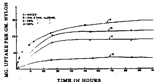
Fig. 14.—Effect of ethyl alcohol on the sorption of salicylic acid (0.15%) by nylon (41.5°C). [From Kapadia, A. J., Guess, W. L., and Autian, J., "Sorption and Diffusion Studies of Salicylic Acid in a Nylon Sheet," to be published.]
