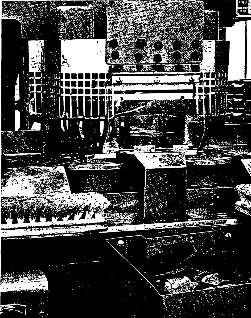
FIG 25-29 – Well guarded double-dial feed Note plastic coating on lower part of metal guard, which eliminates sharp edges and reduces glare
