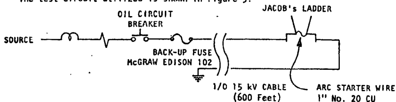
FIGURE 3 TEST CIRCUIT
