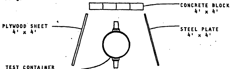
FIGURE 2 TEST SITE
