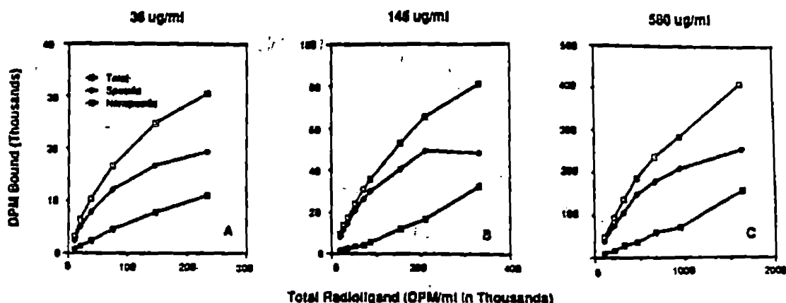
Fig. 2. Equilibrium binding of [ ^{125} I]2-iodo-7,8-dibromodibenzo- p -dioxin. The receptor preparation (ASPPT, 38 (A), 145 (B), or 580 (C) \mu g of protein/ml) was incubated at 4 ^{\circ} for 16 hr, with concentrations of radioligand ranging from 2.5 to 250 fmol/ml. Total, specifically bound, and nonspecifically bound radioligand were determined as outlined in Materials and Methods. Each point represents the average of duplicate determinations.
