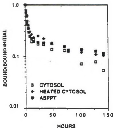
Fig. 9. Dissociations of [ ^{125} I]2-iodo-7,8-dibromodibenzo- p -dioxin from different receptor preparations at 4°C. Dissociation rates were determined as described in Fig. 8. Cytosol (85 µg of protein/ml) and ASPPT (72 µg/ml) were preincubated with 10 pM radioligand for 16 hr at 4°C before dissociation rate determinations. Heated cytosol was preincubated for 18 hr at 4°C as above, followed by a 30-min incubation at 30°C, then recooled to 4°C (30 min) before dissociation rate determination. Kinetic rate constants were calculated by the nonlinear curve fitting technique, constrained to a biexponential model, as described (16).
