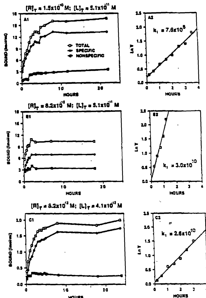
Fig. 6. Time course of association of [^{125}\text{I}]2\text{-iodo-7,8-dibromodibenzo-p-dioxin} to the hepatic Ah receptor at 4^\circ\text{C} : estimate of the association rate constant. The time course of ligand receptor association was monitored at receptor concentrations of 1.5 \times 10^{-10} \text{ M} and 8.2 \times 10^{-12} \text{ M} (ASPPT fraction equal to protein concentrations of 1160 and 72 \mu\text{g/ml} ) and radioligand concentrations of 5.1 \times 10^{-11} \text{ M} and 4.1 \times 10^{-12} \text{ M} (250,000 and 20,000 dpm/ml). Each point represents the average of two determinations. The data are presented as a plot of bound radioligand as a function of time (A1, B1, and C1), and as a plot of \ln Y (left side of Eq. 3) as a function of time (A2, B2, and C2). The rate constant of association was determined from the slope of \ln Y versus time plots as described in Eq. 4 and is inset (units of \text{M}^{-1} \text{ hr}^{-1} ).
