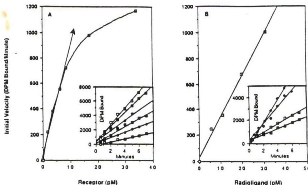
Fig. 7. Initial binding velocity of [ 125 I]2-iodo-7,8-dibromodibenzo-p-dioxin to the hepatic Ah receptor: estimate of the association rate constant. The ASPPT fraction in MDENG buffer was incubated with radioligand in 50-ml Erlenmeyer flasks. At the indicated times intervals, 1.0-ml aliquots were transferred to borosilicate tubes containing 1000-fold molar excess of 2,3,7,8-tetrachlorodibenzofuran (800-fold for nonspecific binding) to prevent further binding of the radioligand and total, specifically, and nonspecifically bound radioligand was determined. Receptor concentrations were determined by duplicate Scatchard analyses. A. Initial binding velocity as a function of Ah receptor concentration. Receptor concentrations of 1.7 \times 10^{-12} M ( \square ), 3.4 \times 10^{-12} M ( \Phi ), 6.1 \times 10^{-12} M ( \square ), 8.5 \times 10^{-12} M ( \diamond ), 1.7 \times 10^{-11} M ( \blacksquare ), and 2.4 \times 10^{-11} M ( \square ) were incubated with a fixed radioligand concentration, 2.7 \times 10^{-11} M. The initial binding velocity was determined for each receptor concentration from the slope of the plot of specifically bound radioligand as a function of time (inset). The initial binding velocities were then plotted as a function of receptor concentration. The rate constant of association was calculated from the slope of the linear portion of the line (asymptote of the hyperbola) divided by the ligand concentration (see Materials and Methods). B. Initial binding velocity as a function of radioligand concentration. A fixed concentration of receptor, 6.8 \times 10^{-12} M, was incubated with radioligand concentrations of 5.6 \times 10^{-12} M ( \square ), 1.1 \times 10^{-11} M ( \square ), 2.0 \times 10^{-11} M ( \Phi ), and 3.1 \times 10^{-11} M ( \square ). The initial binding velocity was calculated from the slope of specifically bound radioligand as a function of time (inset). The initial velocity was plotted as a function of radioligand concentration. The rate constant of association was calculated from the slope of this line divided by the receptor concentration.
