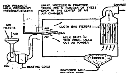
FIG. 15. SPRAY DRYER OF THE PRESSURE-SPRAY ROTARY TYPE 8
