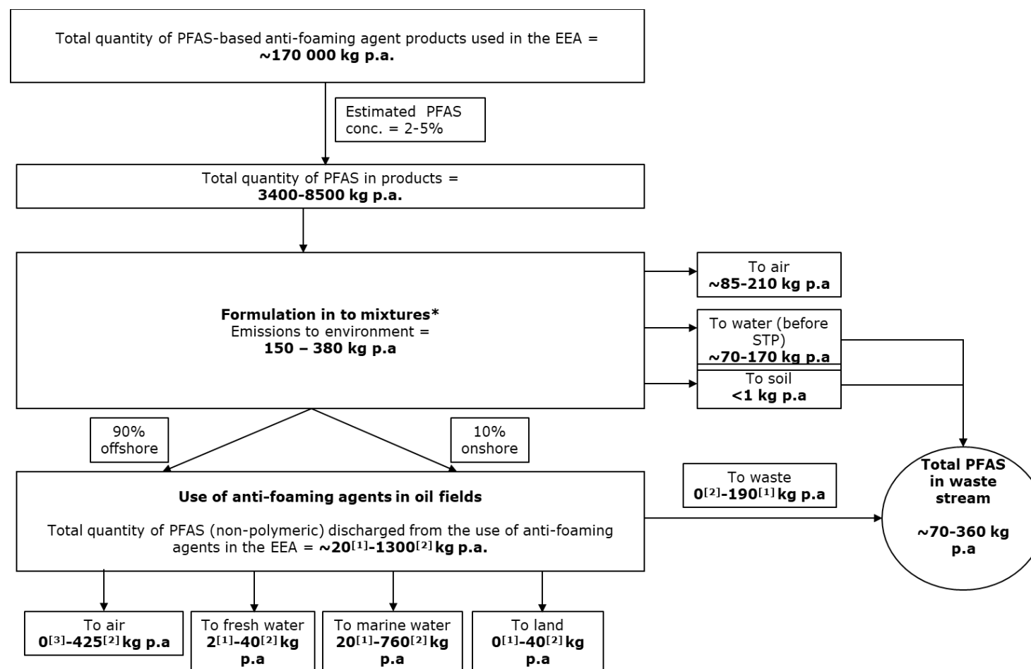
Figure 4-2 Material flow diagram for PFAS (anti-foaming agents)
