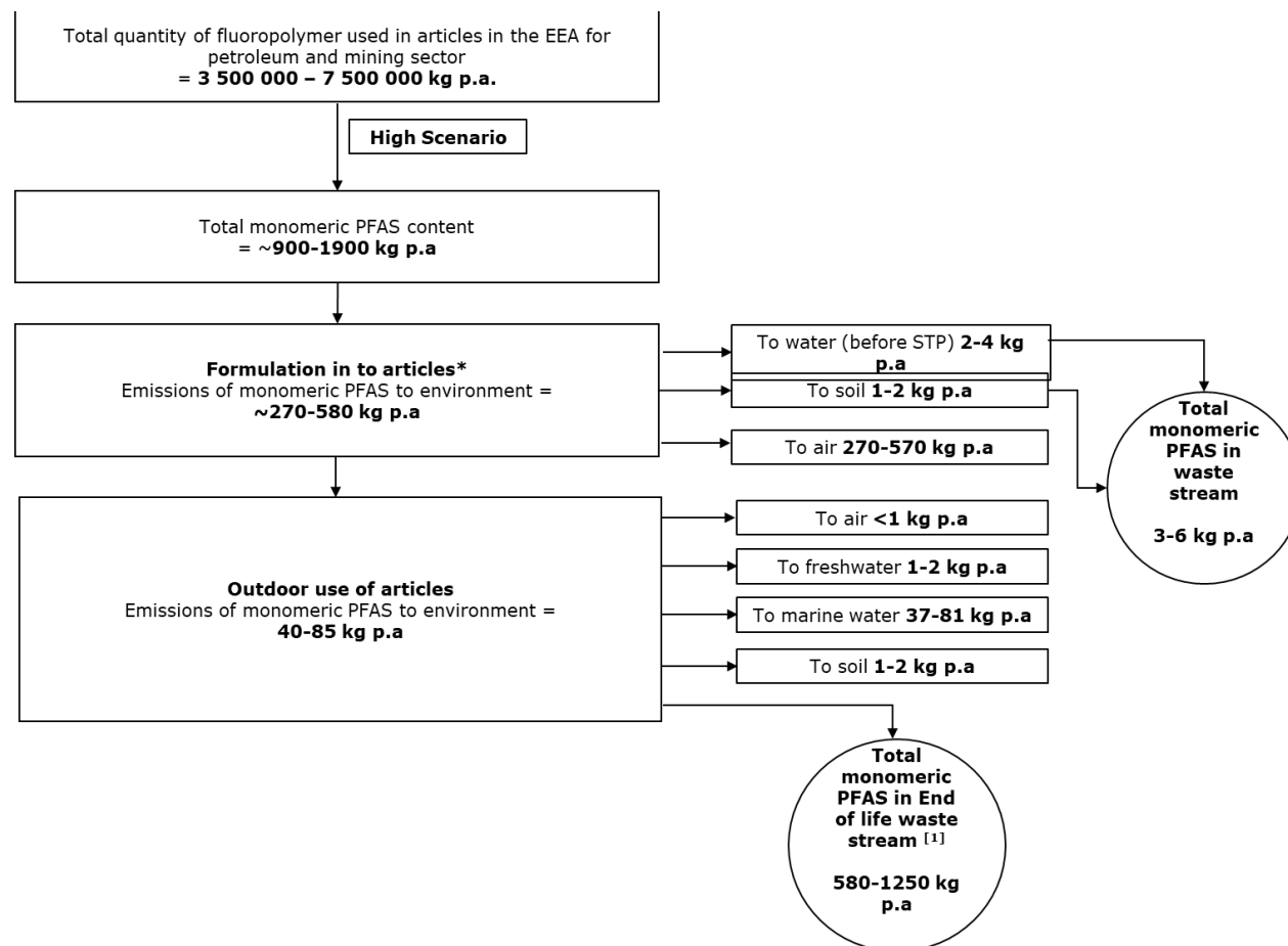
Figure 4-4 Material flow diagram for PFAS (fluoropolymer agents, high scenario)
