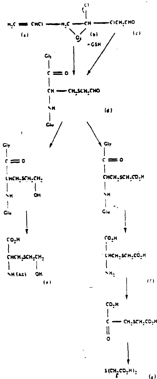
Fig. 1. Scheme showing the metabolism of vinyl chloride monomer (VCM) in rats to S-containing metabolites. VCM (a) is converted to chloroethylenoxide (b) which is transformed spontaneously to chloroacetaldehyde (c). These two metabolites are mutagenic and hence are considered to be the proximate carcinogens. The urinary excretion products N-acetyl-S-(2-hydroxyethyl)cysteine (e) S-(carboxymethyl)cysteine (f) and thiodiglycolic acid (g) are derived from these mutagenic metabolites via (d). Gly and Glu are the glycine and glutamate residues of glutathione. (After Green & Hattaway (1977)).
