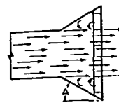
FIG. 8. EFFECTS OF EXPANDING DUCT
