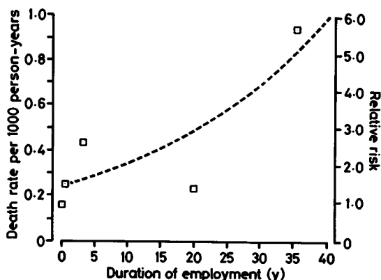
Figure 2 Death rate and corresponding RR from all respiratory cancers (1927–86) v exposure time for 1454 asbestos cement workers and 762 referents (time 0) with a minimum of 20 years latency time. Squares and dashed line are derived from Poisson regression models adjusted for calendar period, age, and duration of employment and are shown for 1947–56 and age group 50–59. Slope estimate is 3.6% (95% CI 1.7–5.5) a year.
