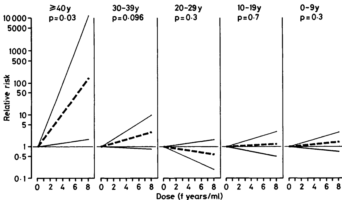
Figure 1 RRs (---) and 95% CIs (—) for cumulative dose estimated in each 10 year period before diagnosis of mesothelioma ( n = 14 ). Estimates were obtained from a conditional logistic regression analysis in which previous and subsequent exposure were adjusted for.
