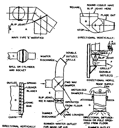
Fig. 3 .... Directional Outlets for Spot Cooling
