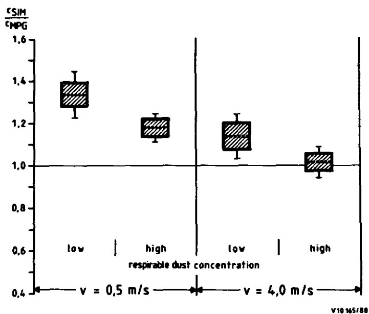
Figure 8. Conversion factors for Simpeds and MPG II.
