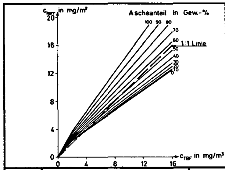
Figure 5. Conversion C_{TBF} into C_{corr} .
