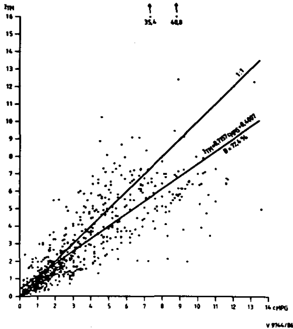
Figure 12. Relation between gravimetric and tyndallometric intensity values of respirable dust concentrations.
