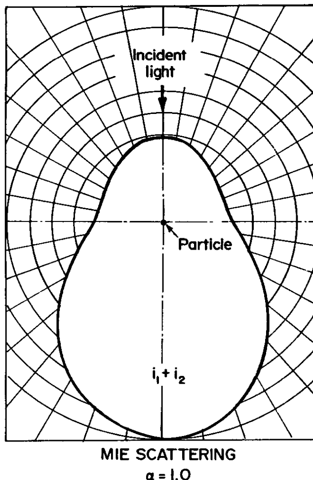
Figure 1. Scattered light intensity as a function of angle \alpha = 1 .
