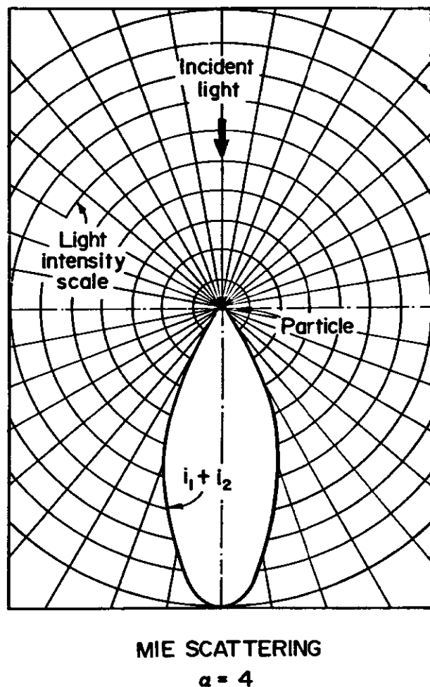
Figure 2. Scattered light intensity as a function of angle \alpha = 4 .
