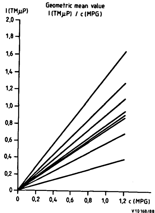
Figure 13. Conversion relation for different faces (low concentrations).
