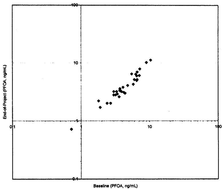
Figure 1. 3M Woodbury Landfill Remediation Project: Baseline vs. End-of-Project PFOA Concentrations (ng/mL).
