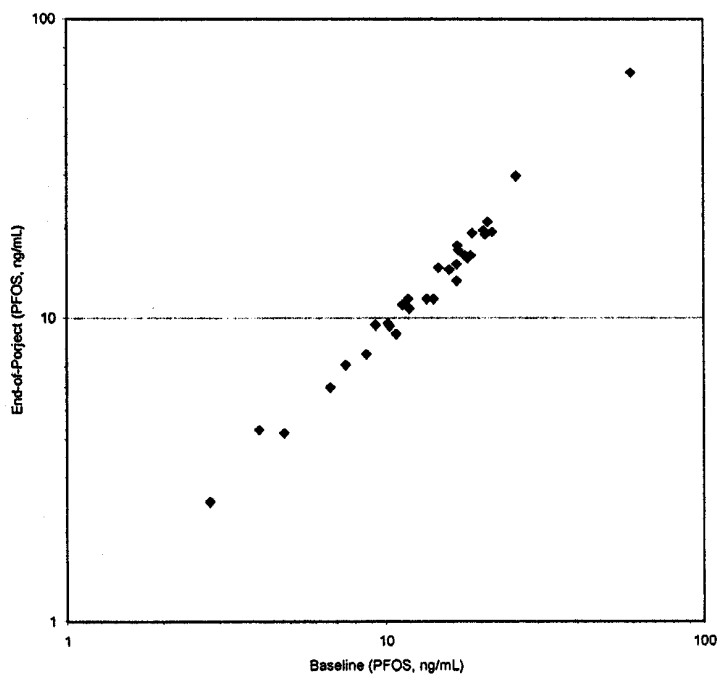
Figure 2. 3M Woodbury Landfill Remediation Project: Baseline vs. End-of-Project PFOS Concentrations (ng/mL).
